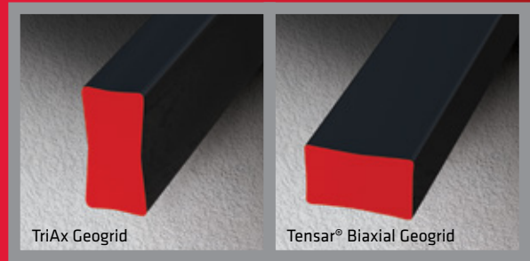
Compared with a conventional biaxial geogrid, TriAx Geogrid has a greater rib depth contributing to improved confinement.
