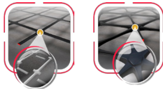
Efficient junctions help to transfer the load applied to a mechanically stabilized layer to the geogrid. If the junctions are not efficient, then the geogrid will not work as effectively.
