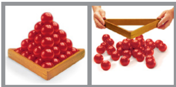
The unique shape of the geogrid ribs confines aggregate particles due to its high stiffness and the strength at the corners (junctions), just like a rack confines billiard balls.
