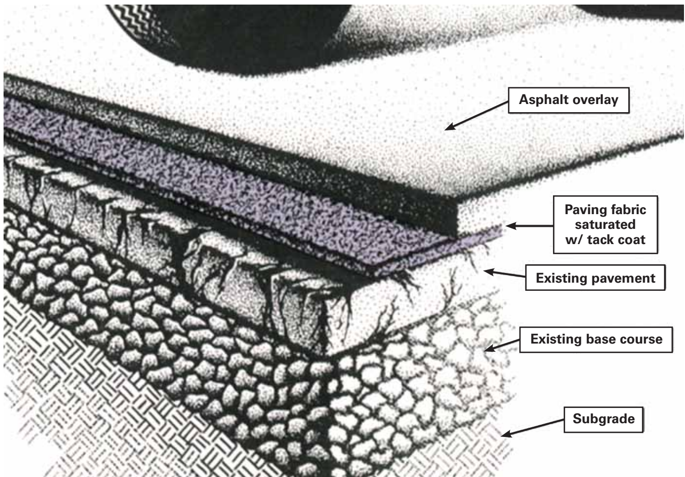
| This diagram illustrates the components of a paving fabric/overlay installation.
